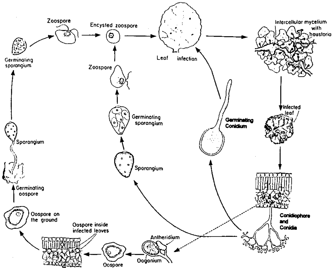
Figure 1 Disease cycle of lettuce downy mildew caused by Bremia lactucae .
